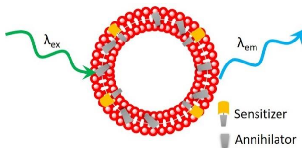
Scheme 1: TTA-UC in liposome containing sensitizer and annihilator under 532 nm excitation.
